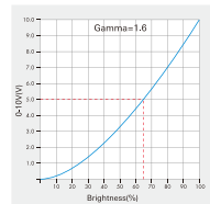
Logarithmic dimming curve
