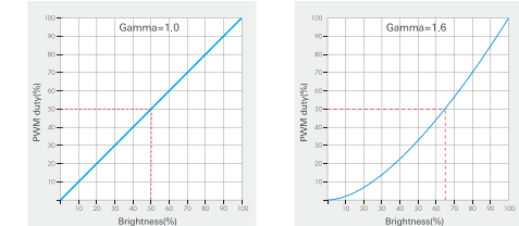
Linear dimming curve Logarithmic dimming curve
